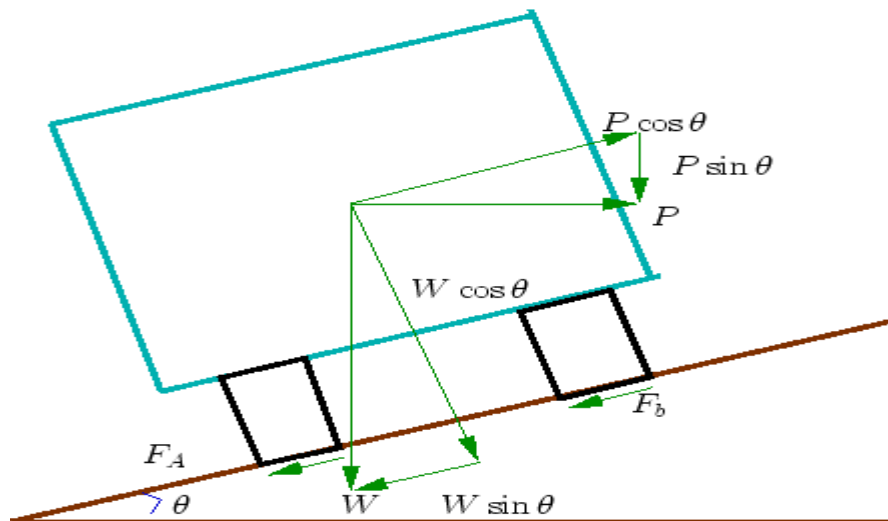
Figure 1: Analysis of super-elevation
