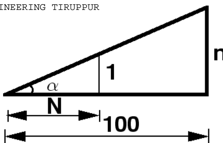
Figure 1: Representation of gradient
