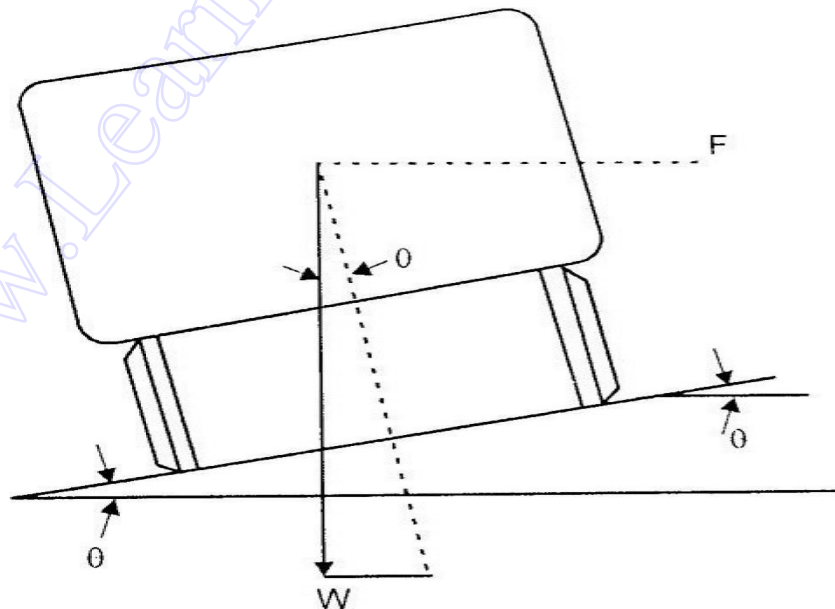
Equilibrium Superelevation
