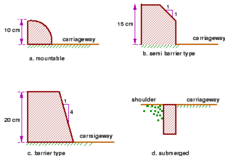
Figure 1: Different types of kerbs
