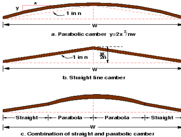
Figure 1: Different types of camber
